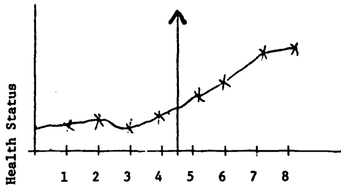
Hypothetical Representation of A Non-Stationary Time Series
